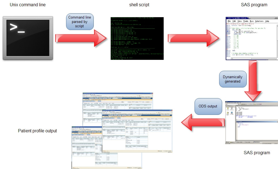
Figure 1. Program diagram. Patient profiles are created using a shell script to parse a command line.
